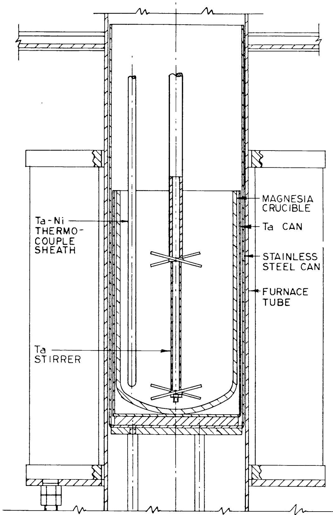
Fig. 3. DOR equipment.
